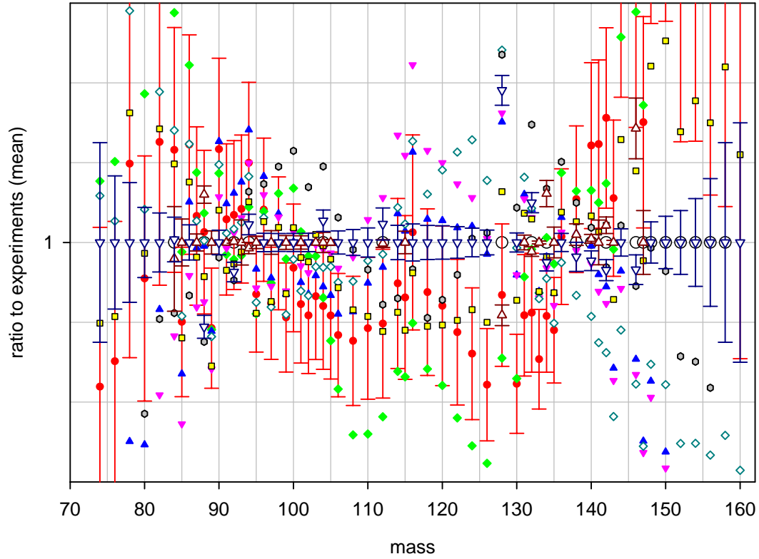
Benchmark A: ^{238}\text{U} at 20-22 MeV, post neutron emission yield ratios to adopted experimental data Lower graph: partial detailed plot (very high and low values omitted), for legend see upper graph.
